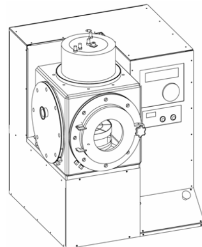
NPE-3000 Table Top PECVD System
